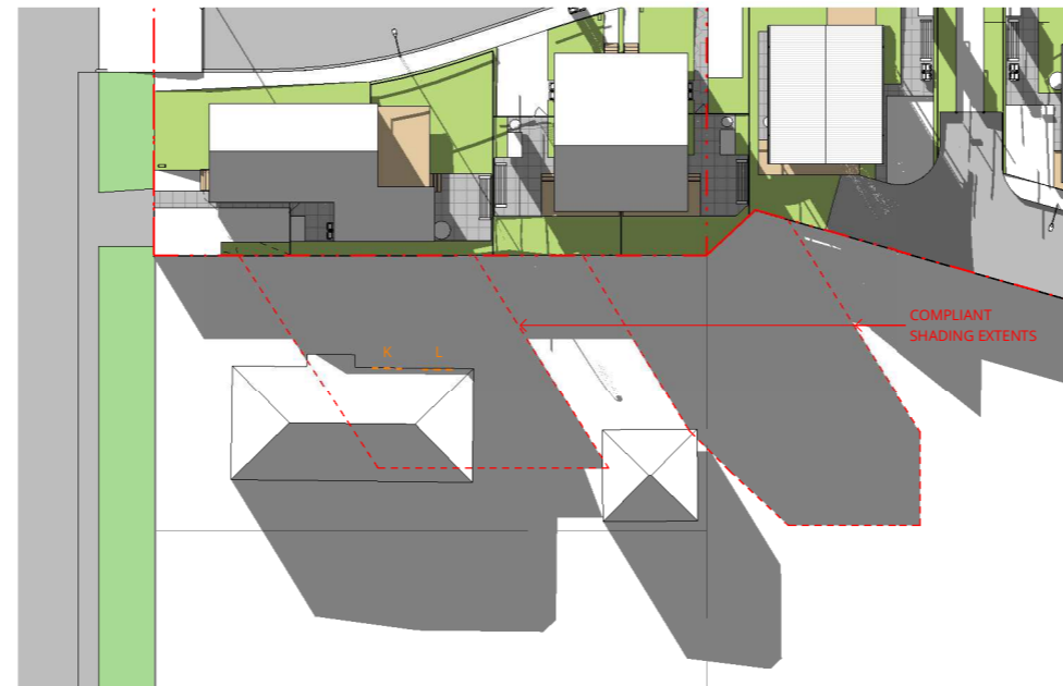
2 SHADING - 21 JUNE - 16.00 COMPLIANT SCALE @ A1: 1 : 300
