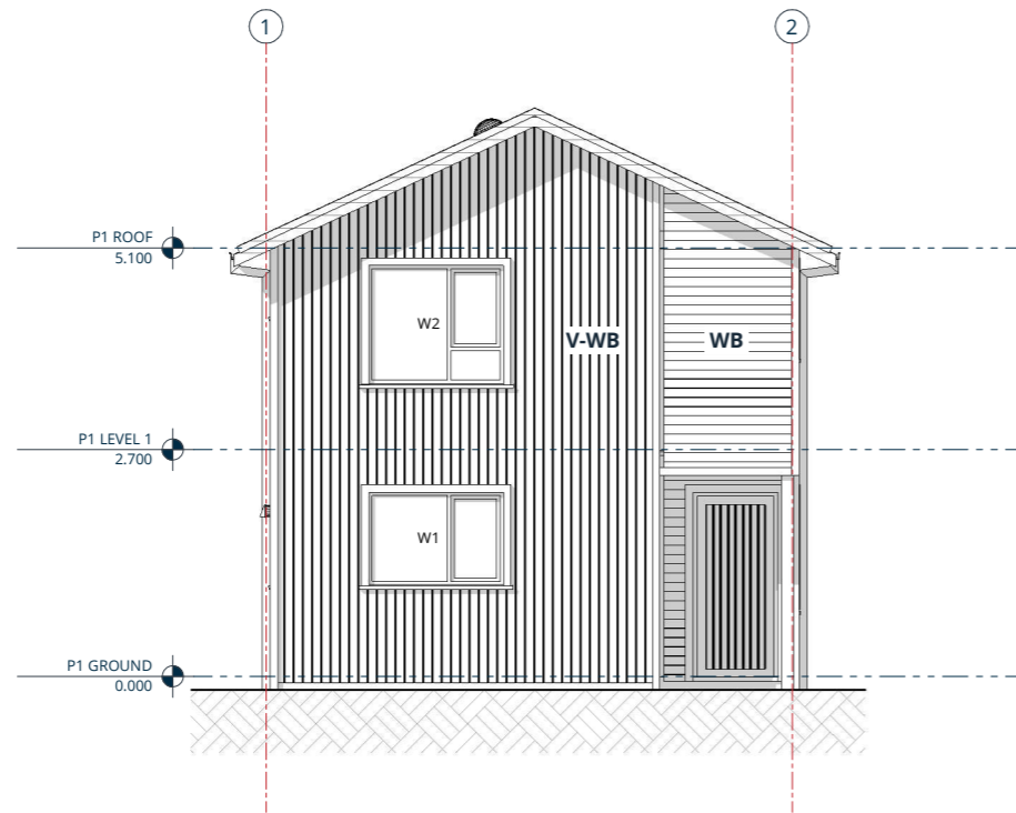
1. FRONT ELEVATION
