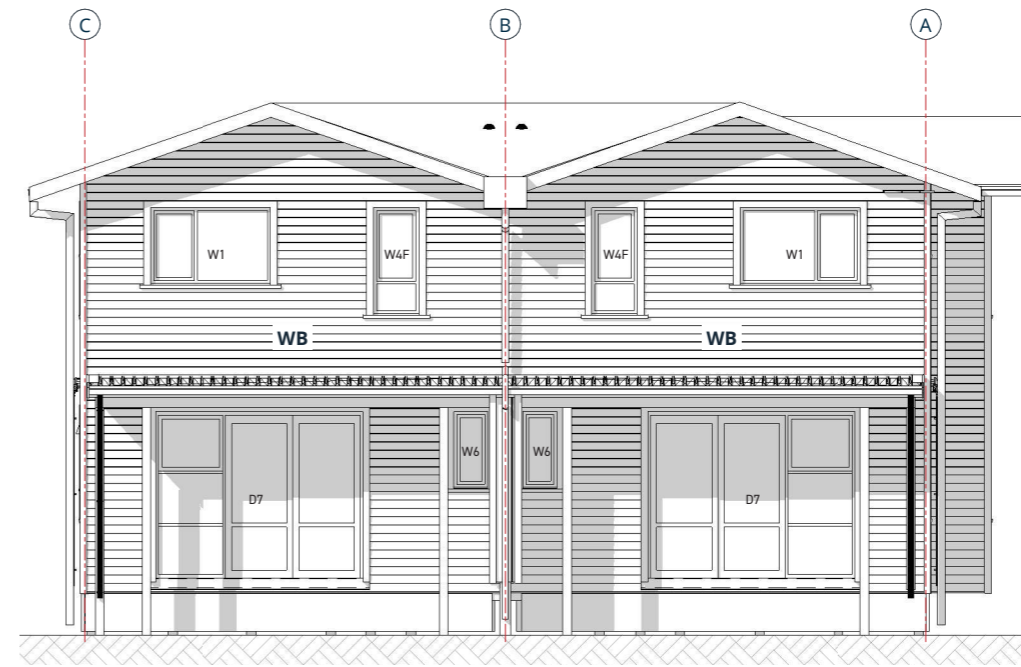
2. REAR ELEVATION
