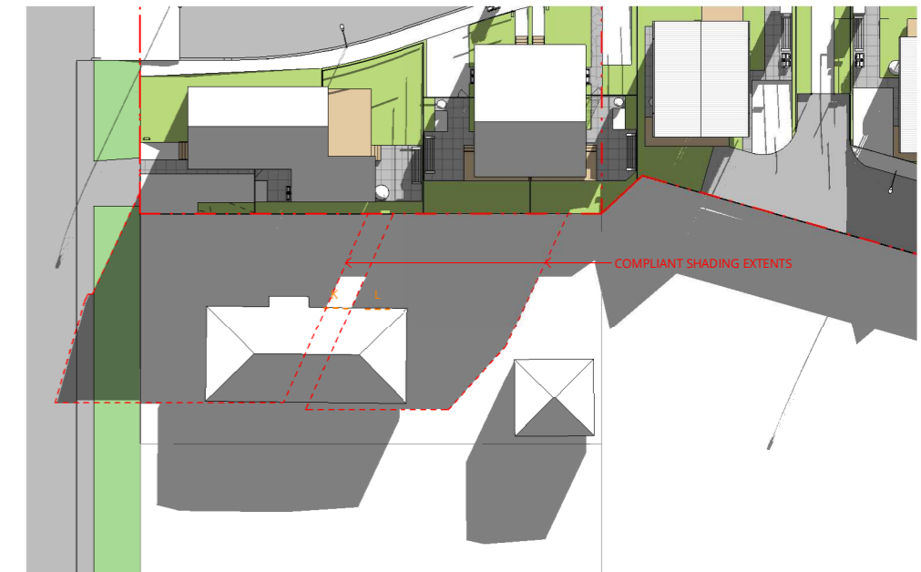
3 SHADING - 21 JUNE - 12.00 COMPLIANT SCALE @ A1: 1 : 300
