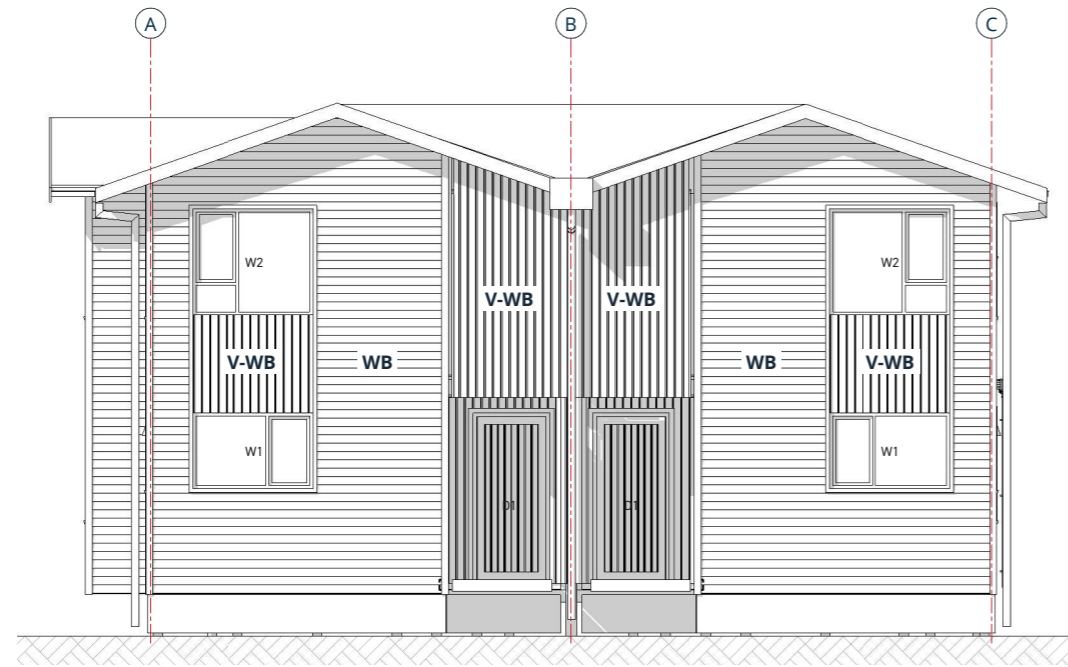
1. FRONT ELEVATION
