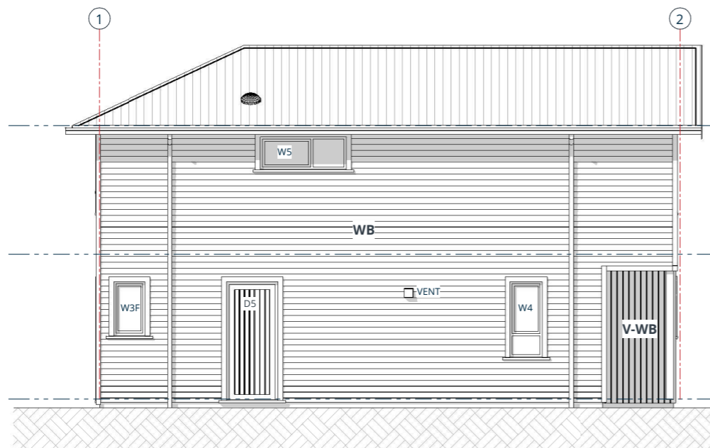
3. LEFT SIDE ELEVATION
