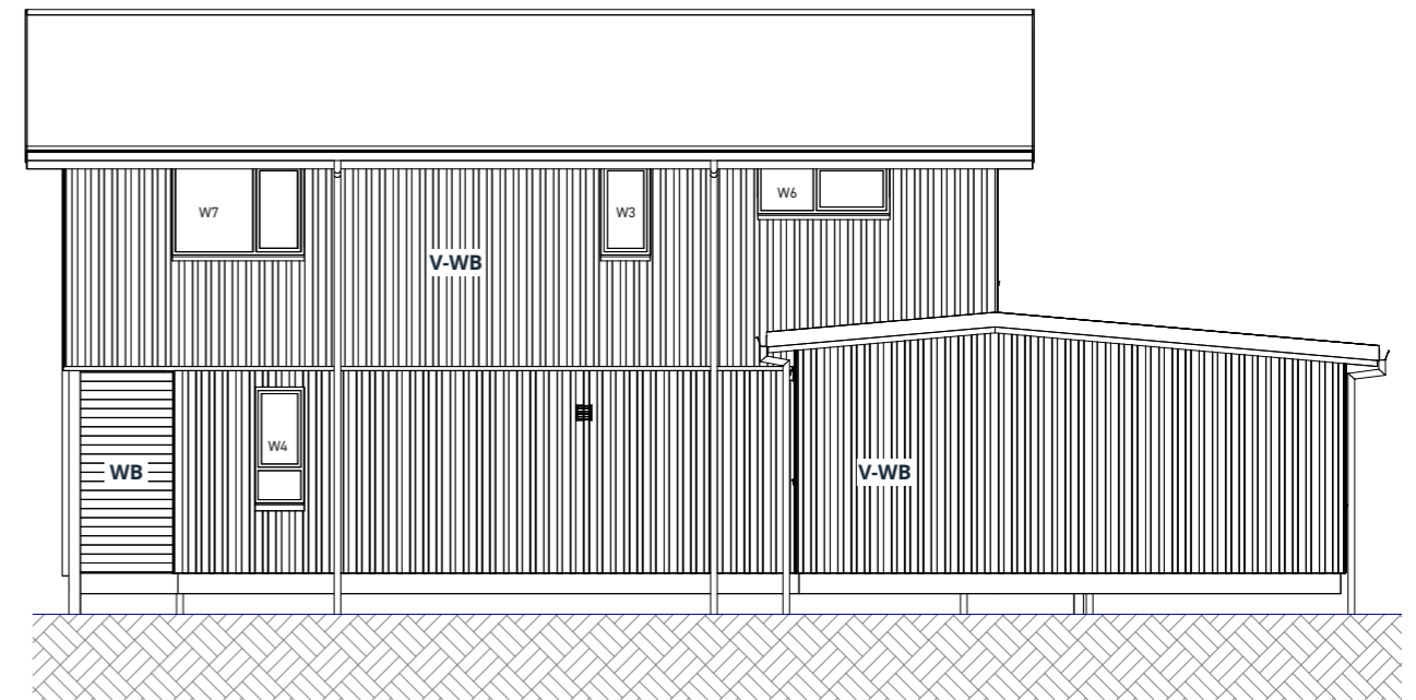
4. RIGHT SIDE ELEVATION
