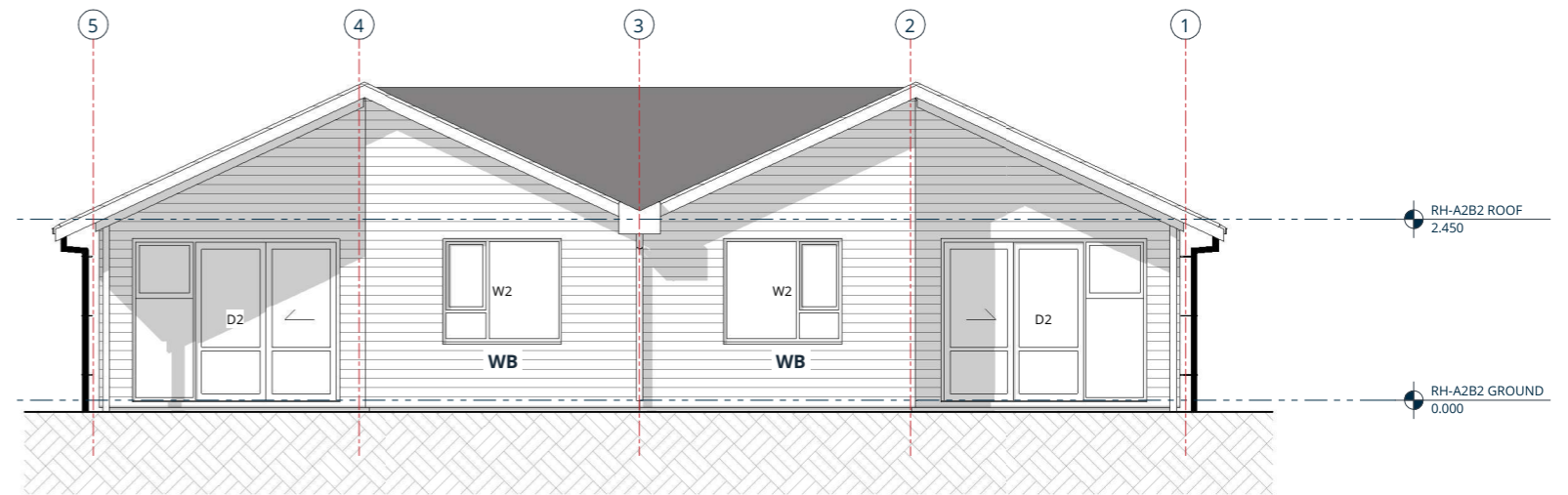
2. REAR ELEVATION
