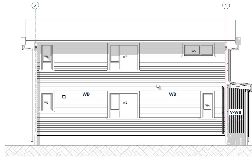
4. RIGHT SIDE ELEVATION
