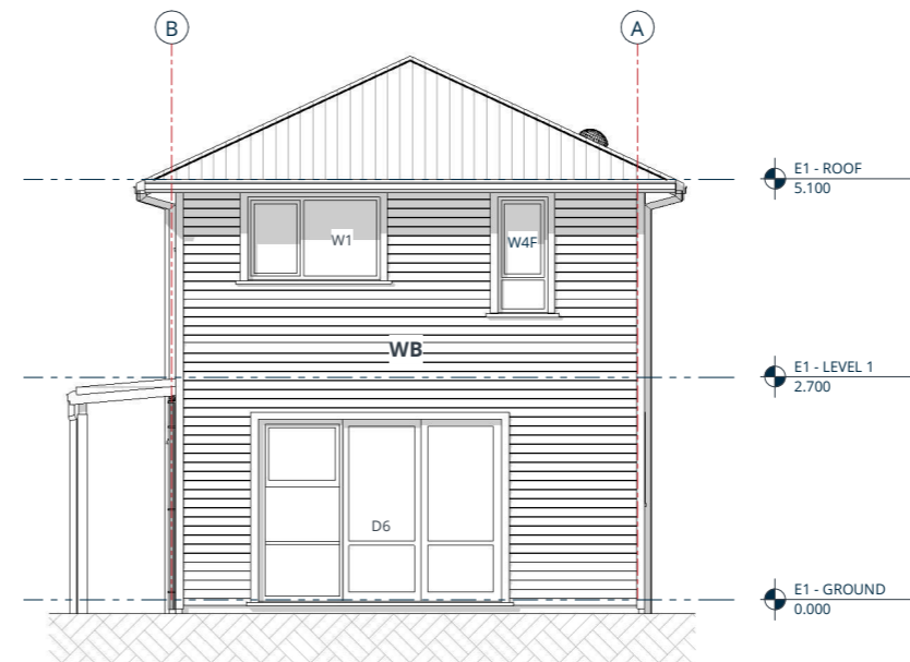
2. REAR ELEVATION
