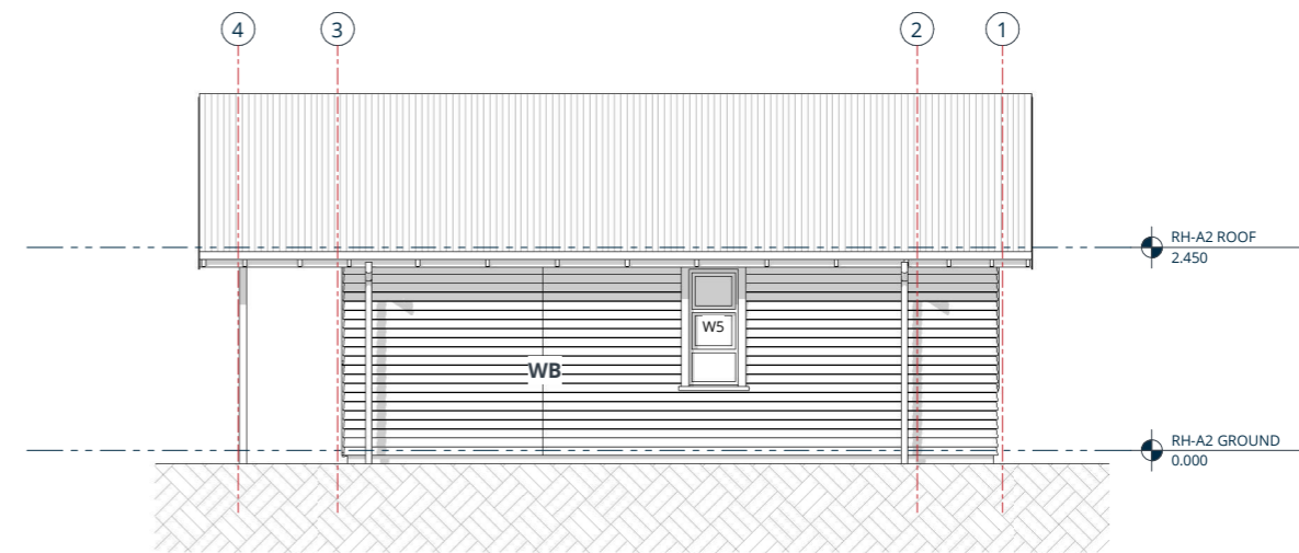
4. RIGHT SIDE ELEVATION
