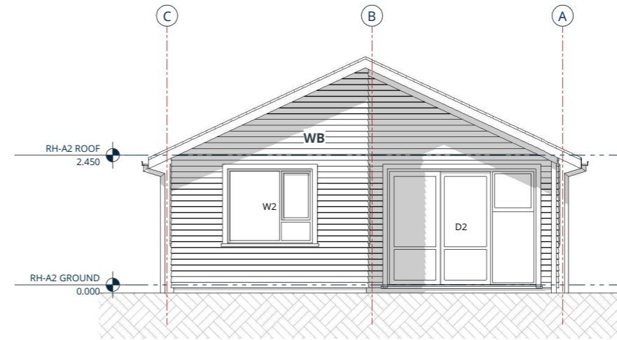
2. REAR ELEVATION
