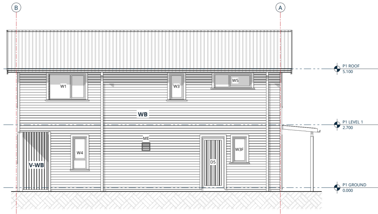
4. RIGHT SIDE ELEVATION
