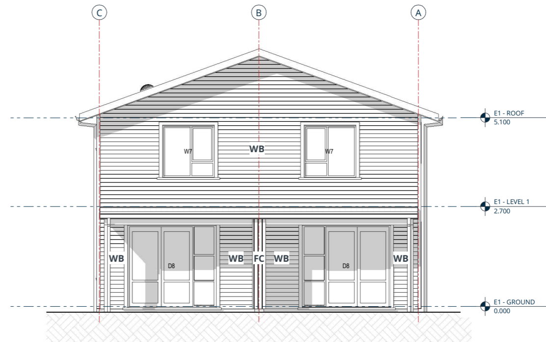
2. REAR ELEVATION
