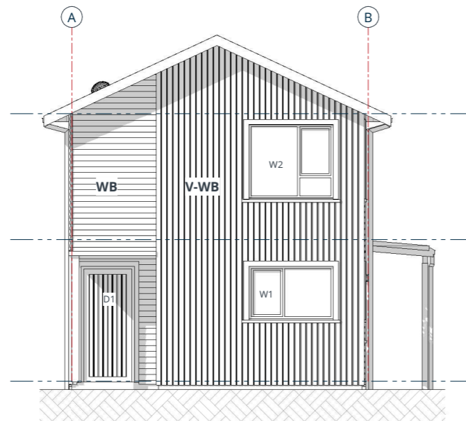
1. FRONT ELEVATION
