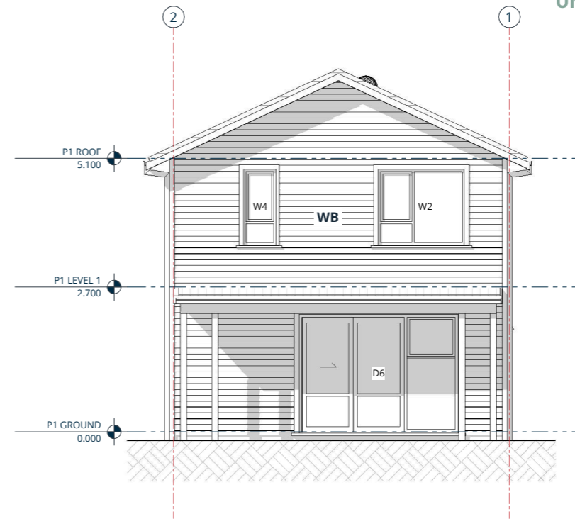
2. REAR ELEVATION
