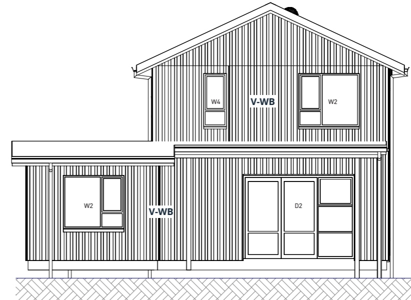
2. REAR ELEVATION
