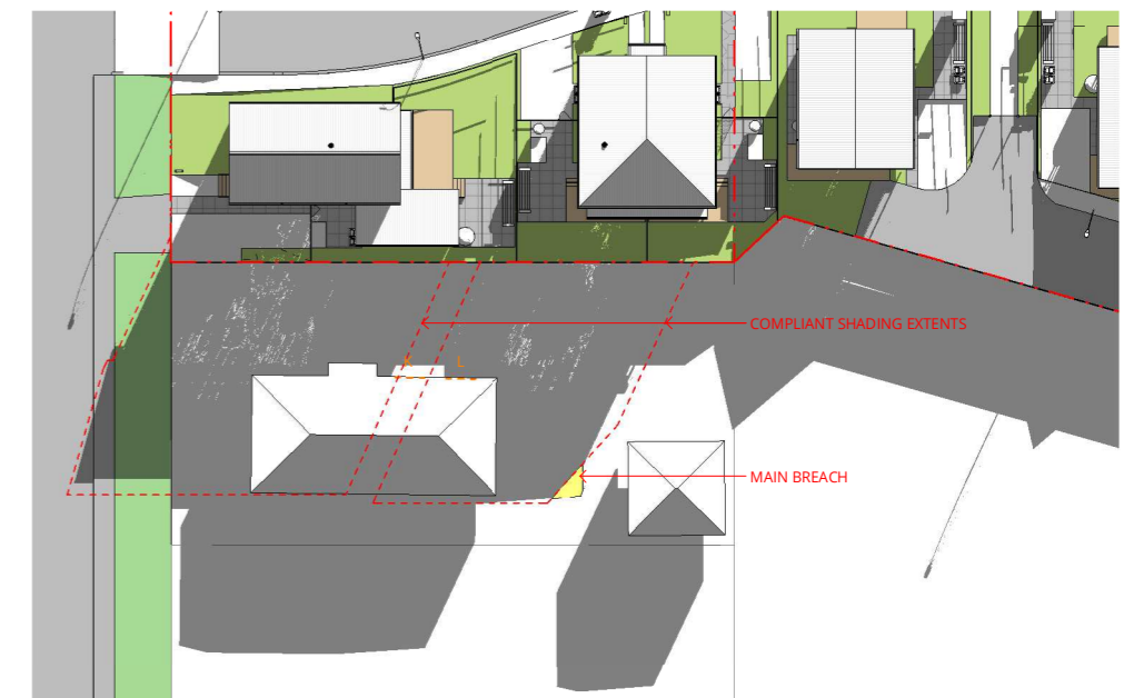
9 SHADING - 21 JUNE - 12.00 PROPOSED SCALE @ A1: 1 : 300
