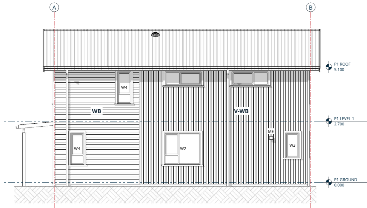
3. LEFT SIDE ELEVATION
