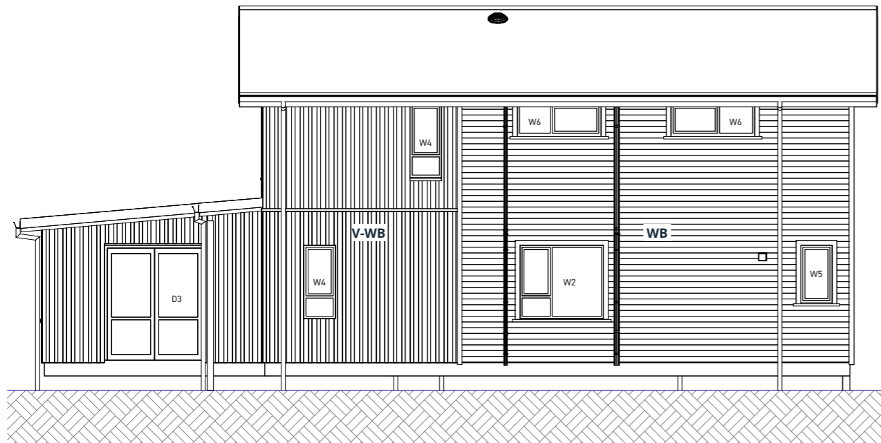
3. LEFT SIDE ELEVATION
