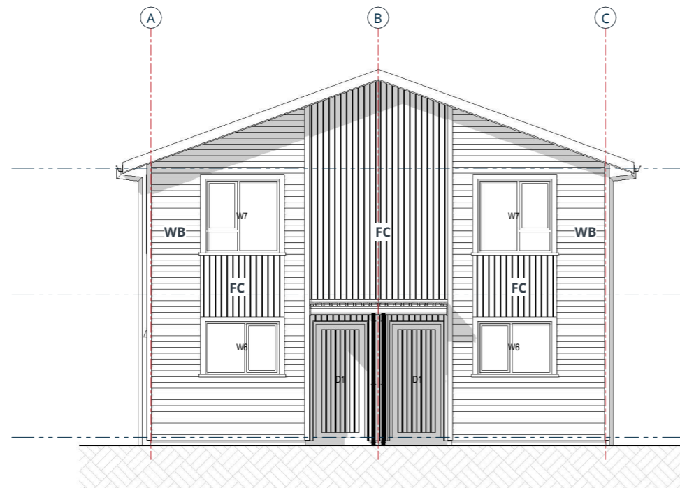
1. FRONT ELEVATION
