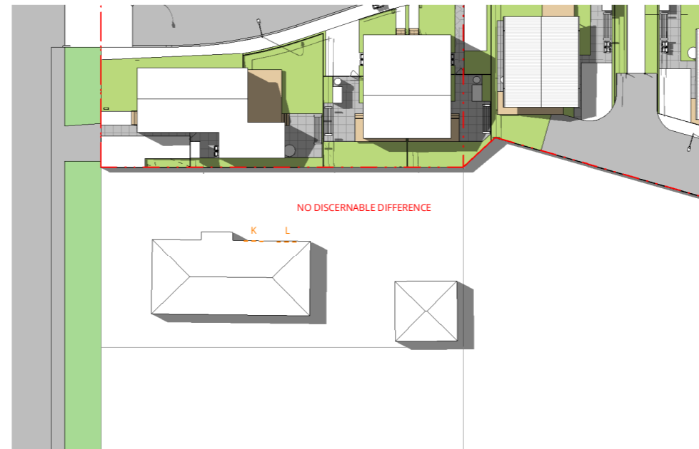
2 SHADING - 21 DEC - 16.00 COMPLIANT SCALE @ A1: 1 : 300
