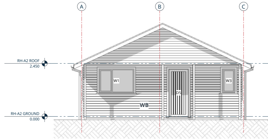
1. FRONT ELEVATION
