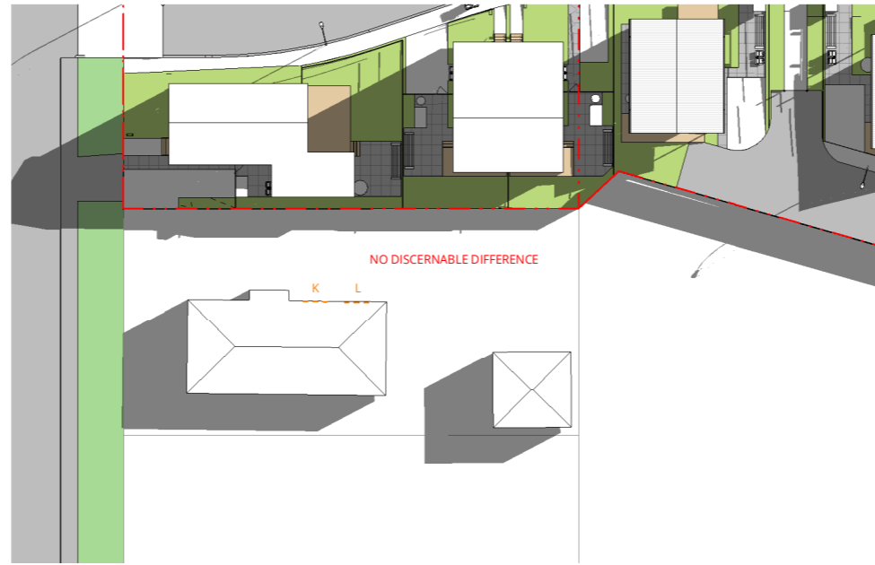
2 SHADING - 21 SEPT - 10.00 COMPLIANT SCALE @ A1: 1 : 300
