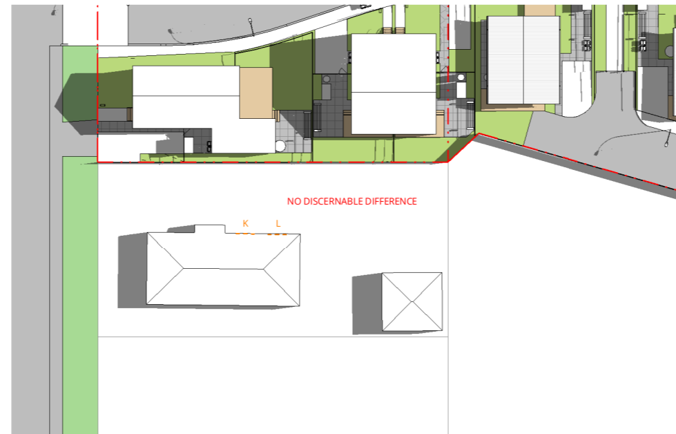
2 SHADING - 21 DEC - 10.00 COMPLIANT SCALE @ A1: 1 : 300
